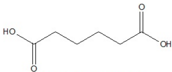
1,4-butanedicarboxylic acid
